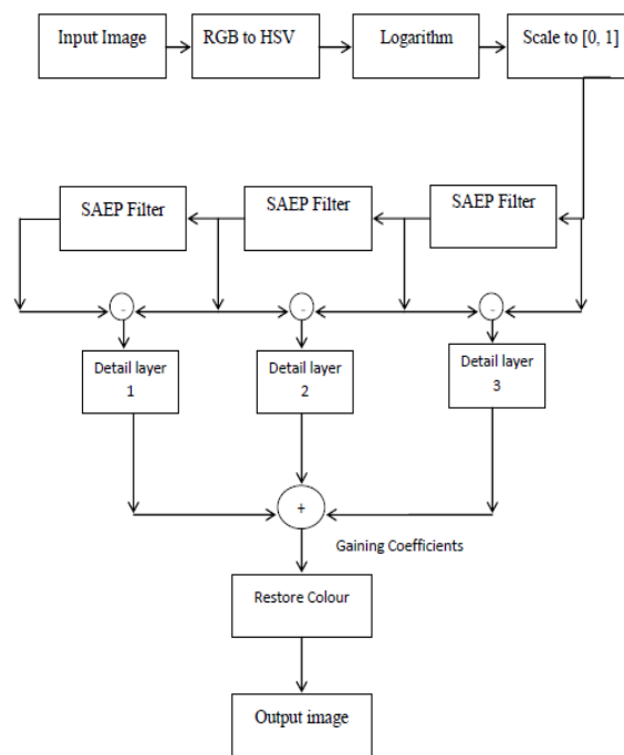
Figure 2: SAEP HDR Tone mapping block diagram
