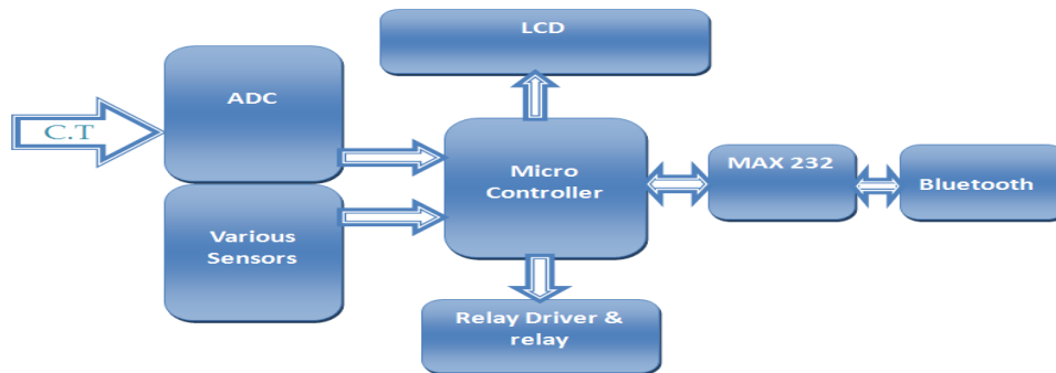
Fig. 3. Block diagram of Agent
