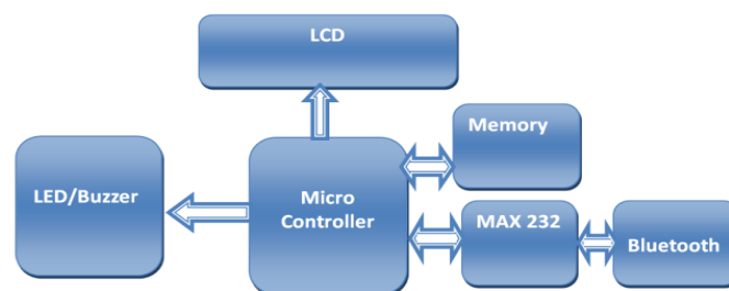
Fig. 2. Block diagram of Host
