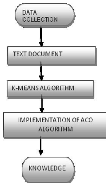
Fig.3 Clustering process
