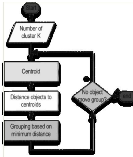
Fig.2. K-Means process
