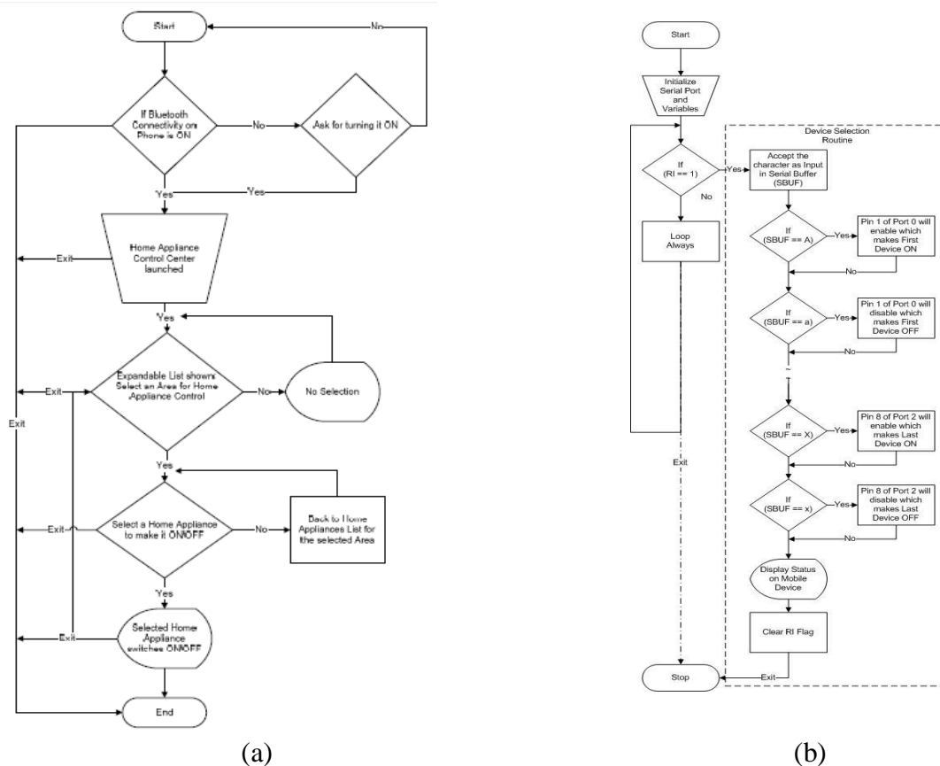
Figure 5. Flow Chart: (a) Android Mobile Application Program (b) Microcontroller Program
