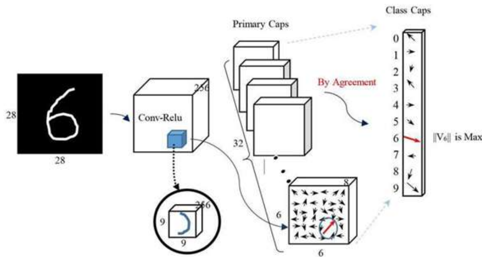
Fig1. Caps Net Architecture
