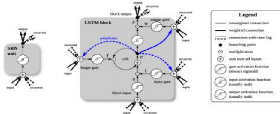
Fig7. LSTM Recurrent Neural Networks
