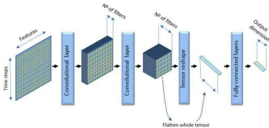
Fig6. Deep Learning in CNN
