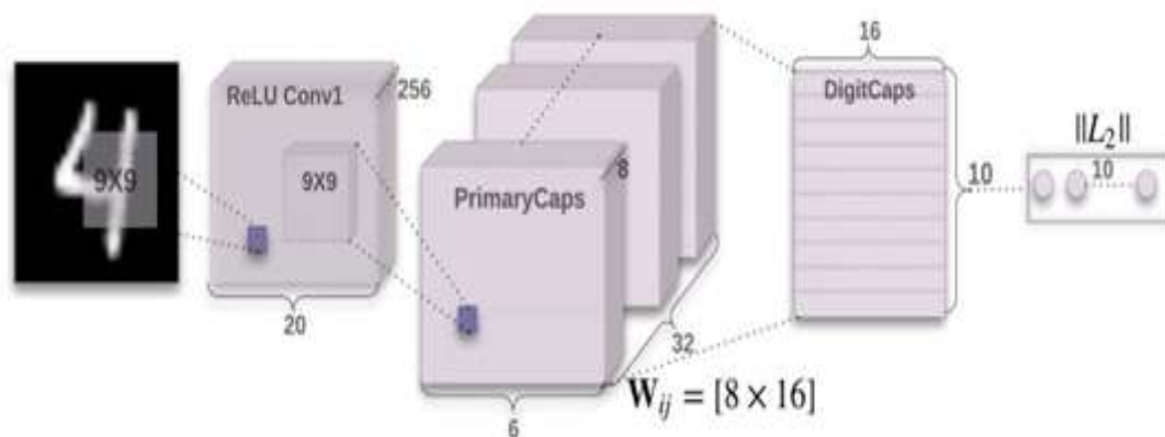
Fig5. Caps Net Neural Network
