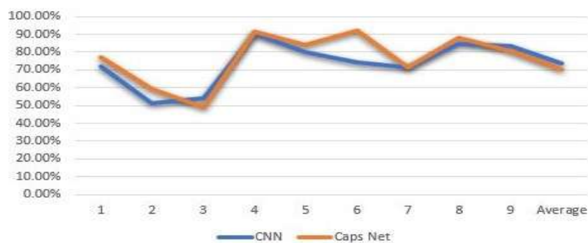
Fig9. Comparison between the CNN and CapsNet
